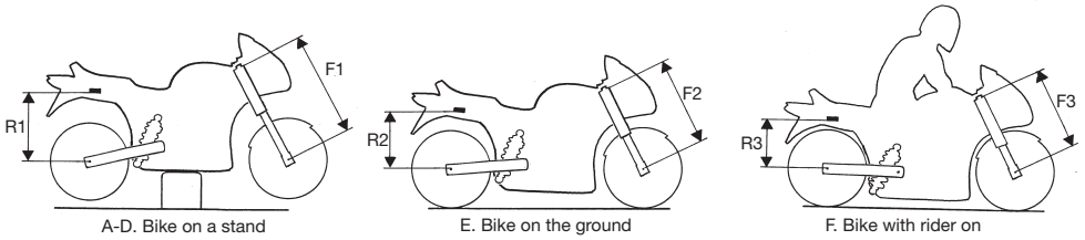
A-D. Bike on a stand
