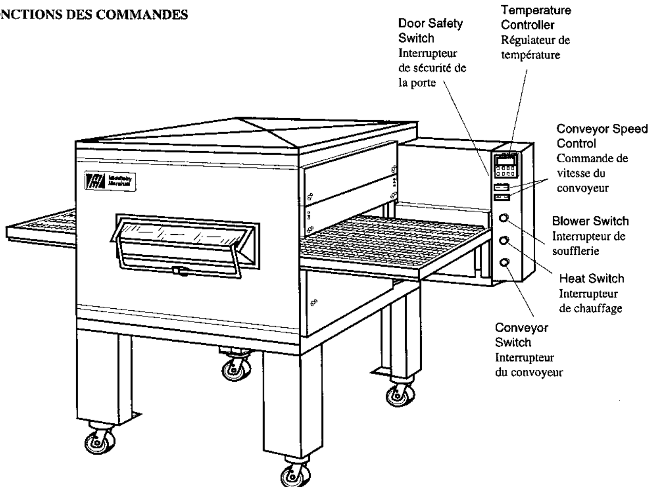
Figure 3-1. PS200-Series Oven Control Functions
