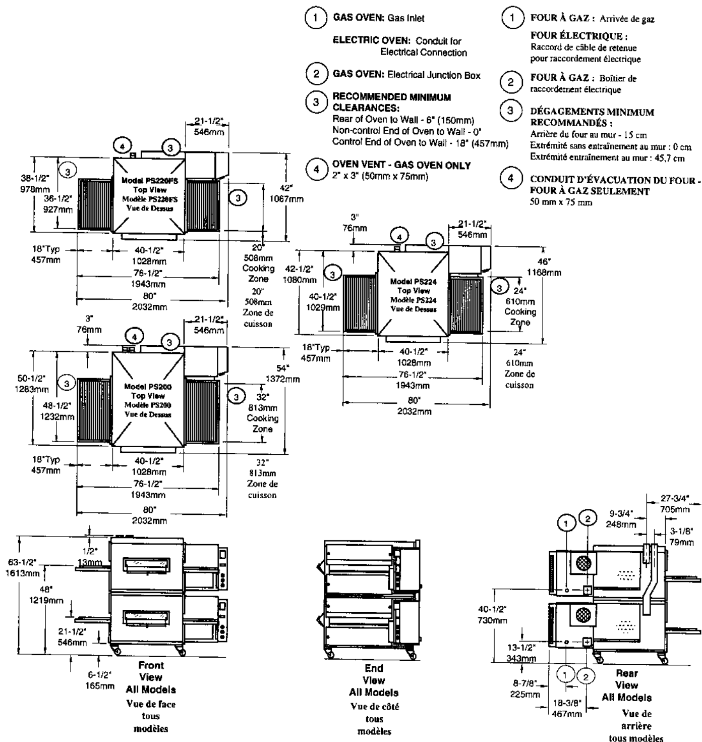
Figure 2-8 SERIES PS200 DOUBLE OVEN DIMENSIONS Figure 2-8. MODÈLES PS200 FOUR DOUBLES - DIMENSIONS
