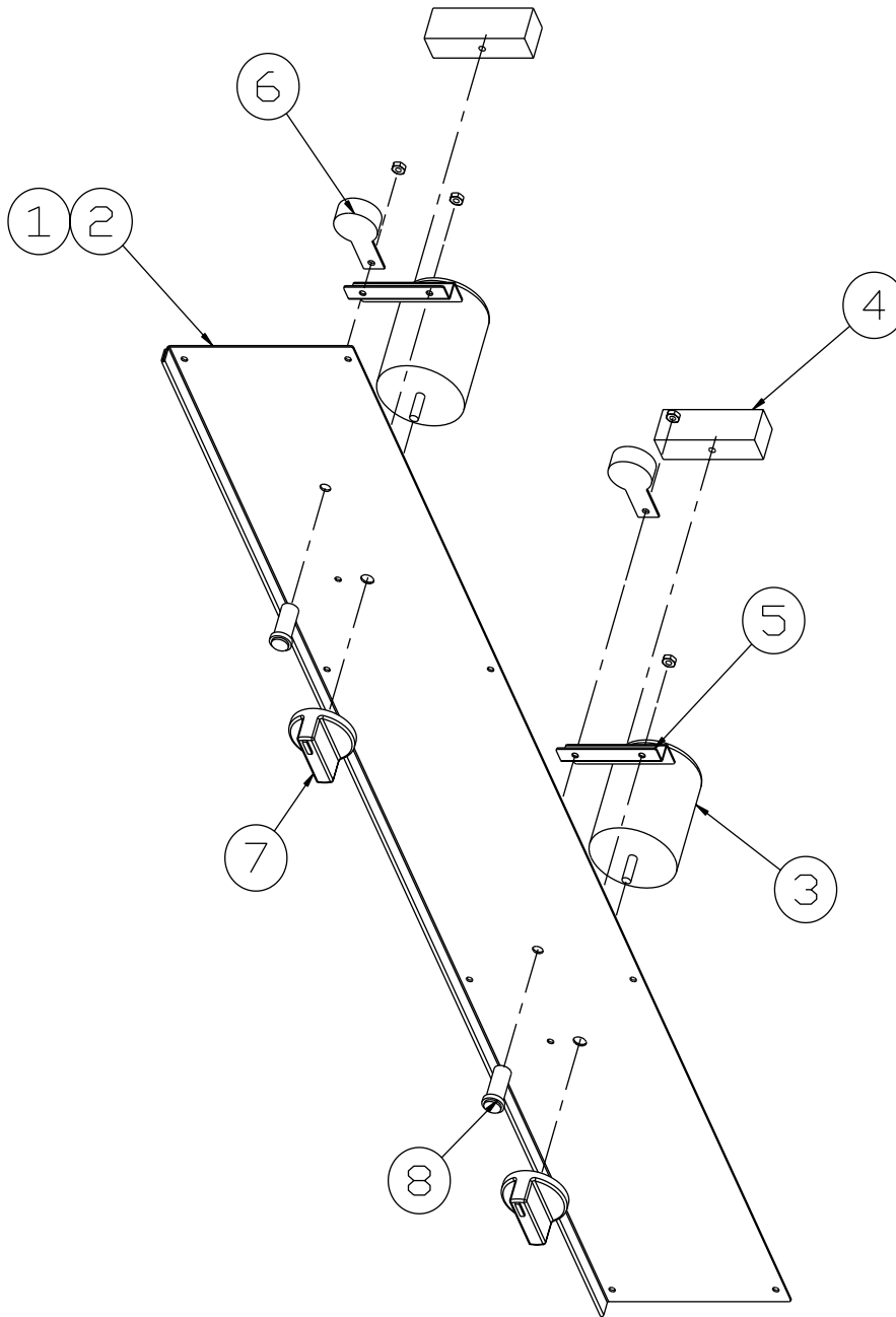
Fig. 6 Control Panel Assembly
