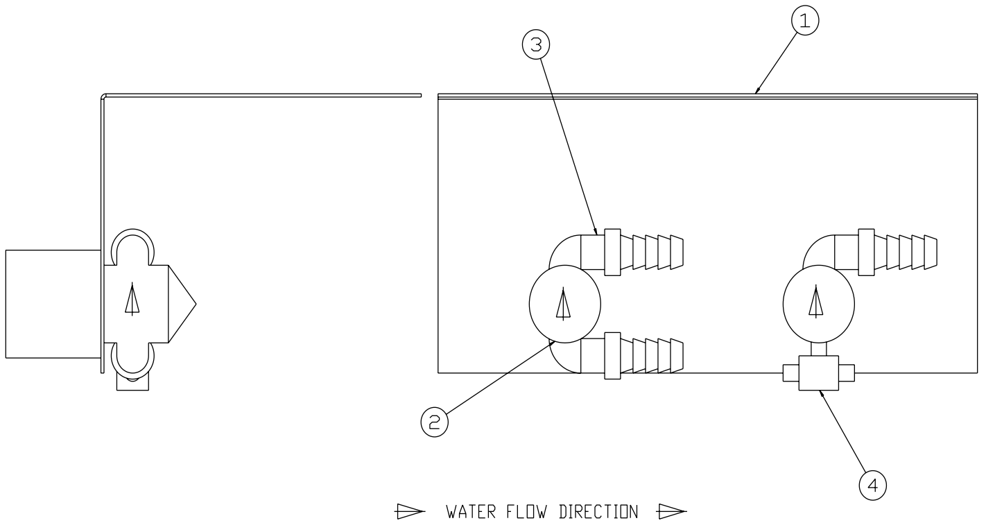
Fig. 7 Condenser Assembly
