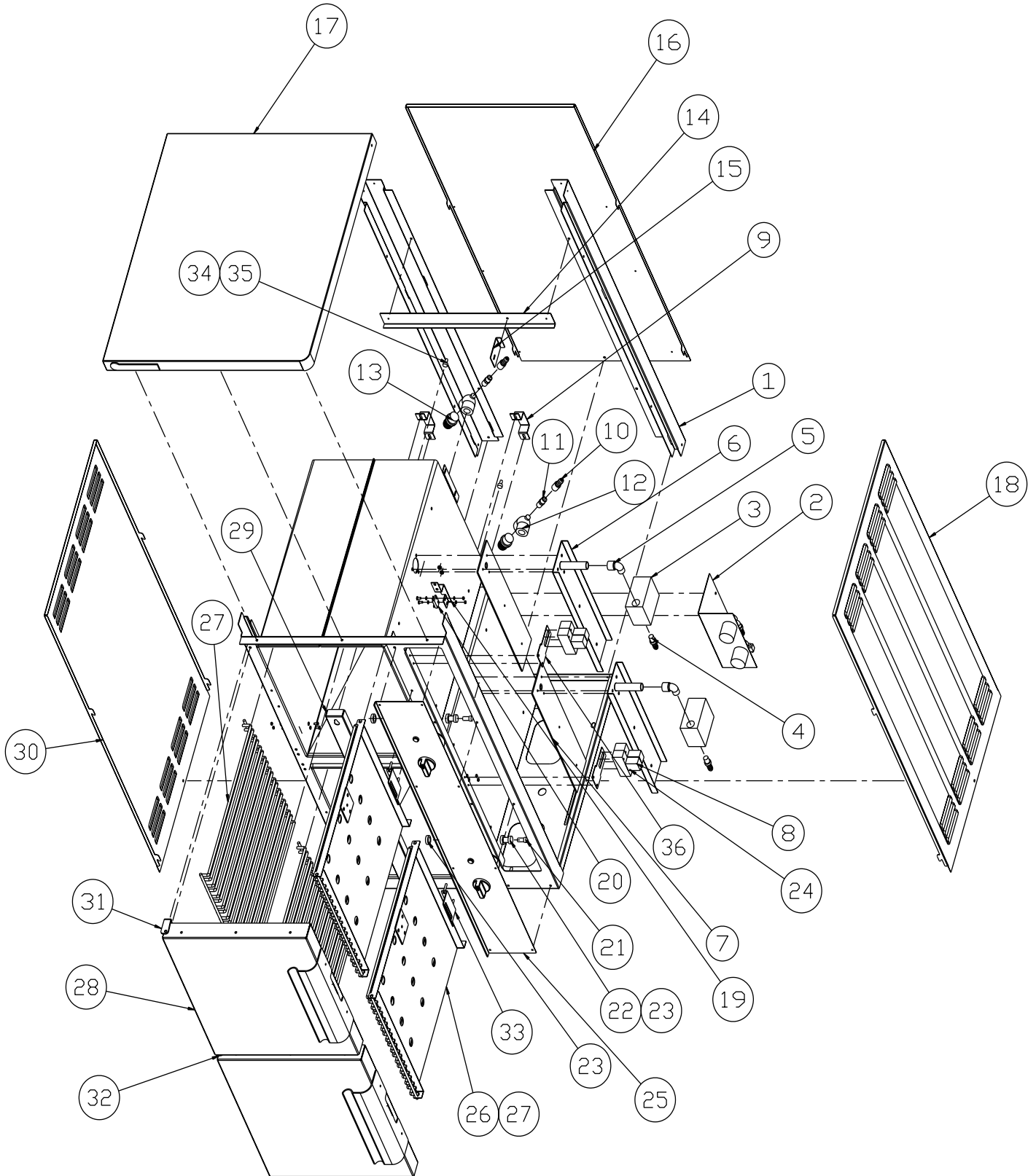
Fig. 4 Cabinet Assembly
