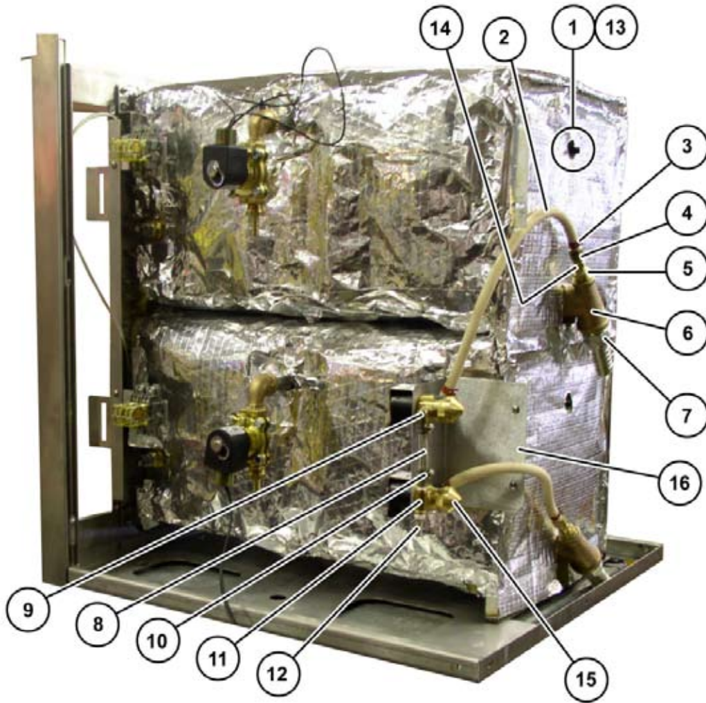
Fig. 8 Complete Condenser Assembly
