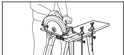
Fig. 4 A typical illustration of proper hand support and workpiece support.
