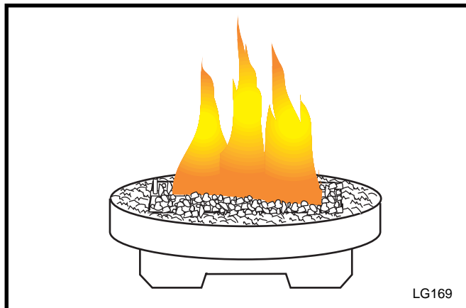
Fig. 17 Correct burner flame appearance.
