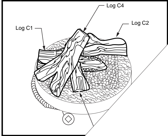
Fig. 13 Logs C3 & C4 place
