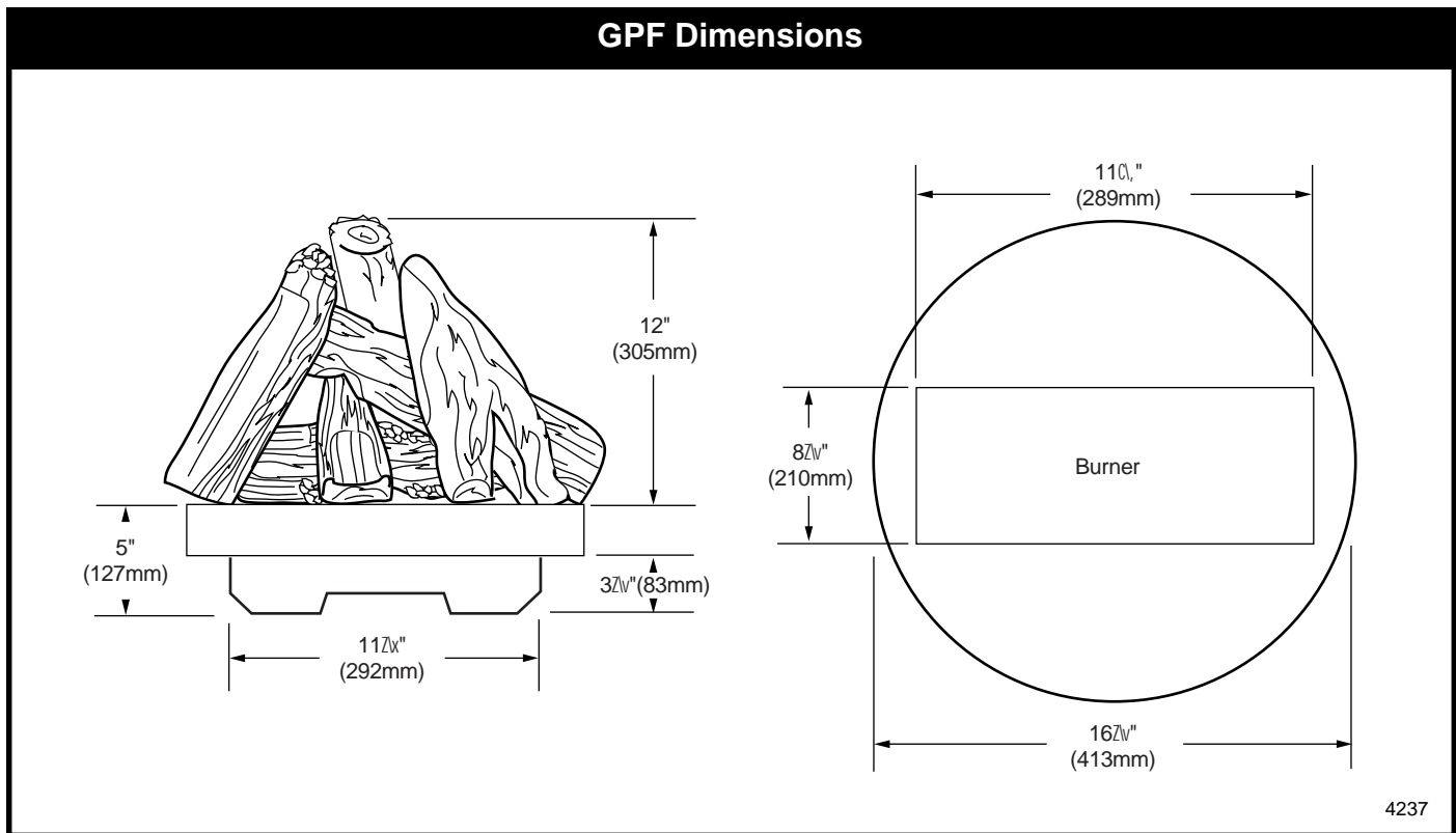
Fig. 1 Physical dimensions.
