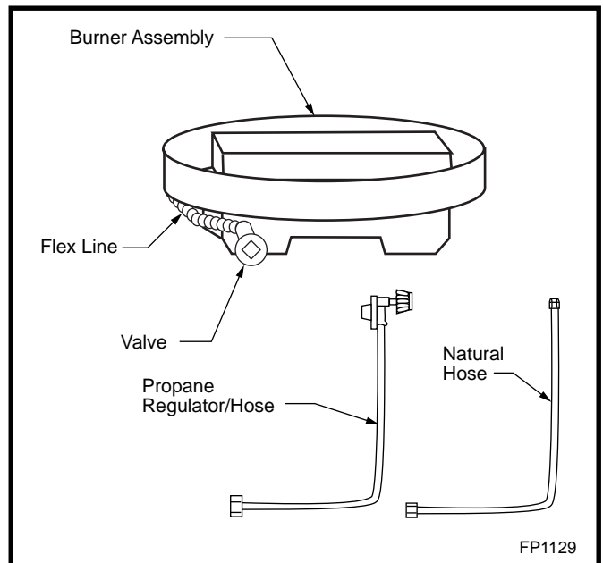
Fig. 2 GPF parts.
