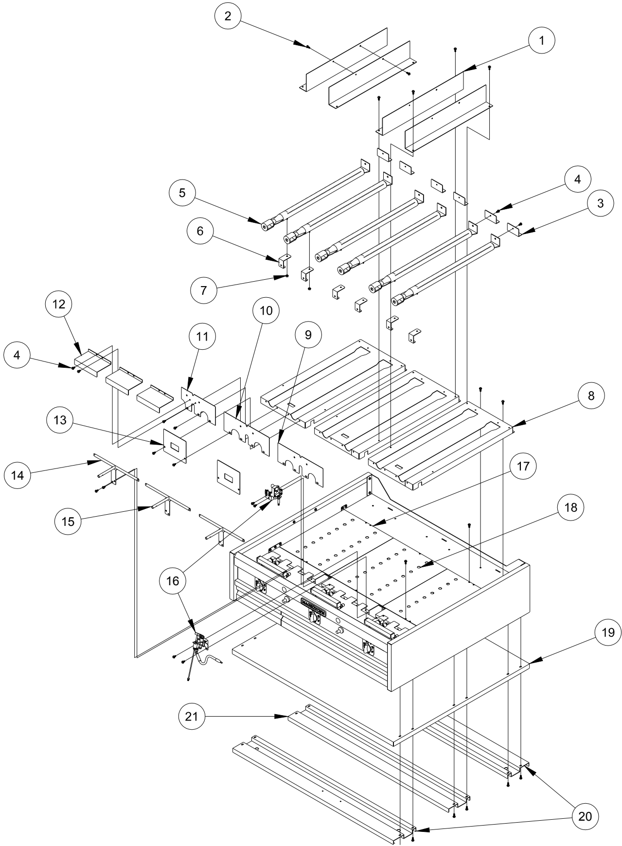
Griddle Assembly Exploded View A1
