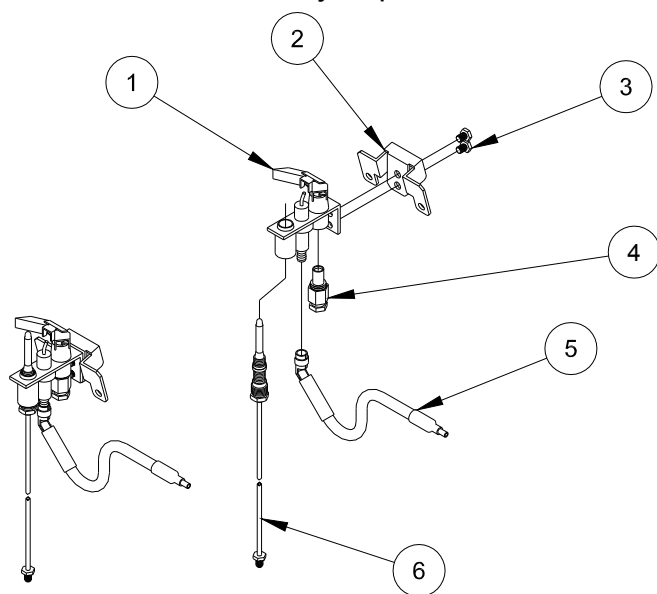
Pilot Assembly Exploded View D2
