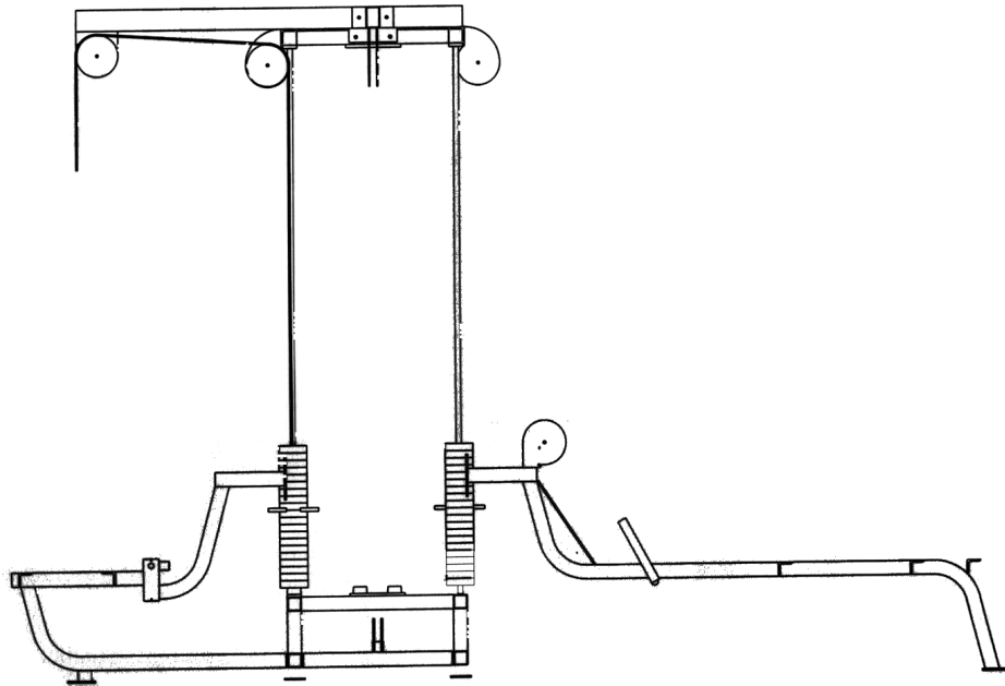
Figure 19. Lat pulldown cable routing.
