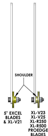
GUIDE WHEEL INSTALLATION (NOTE SHOULDER ORIENTATION)
