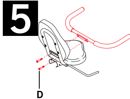
STEP 5: ATTACH HANDLEBAR SET
