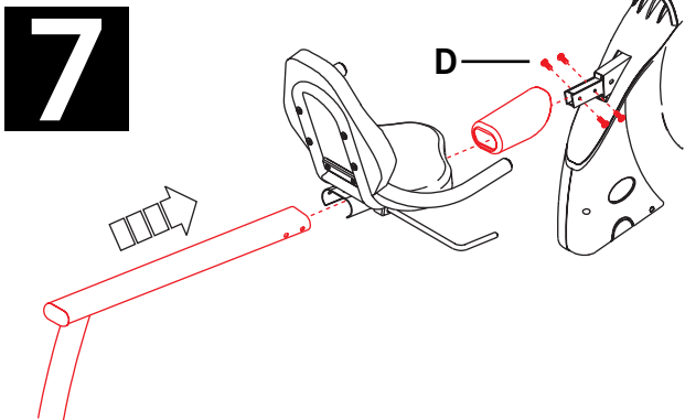
STEP 7: ATTACH SEAT RAIL AND SEAT BOOT
