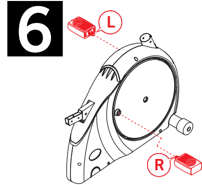
STEP 6: ATTACH LEFT FOOT PEDAL (TURN COUNTER CLOCKWISE) AND ATTACH RIGHT FOOT PEDAL (TURN CLOCKWISE)
