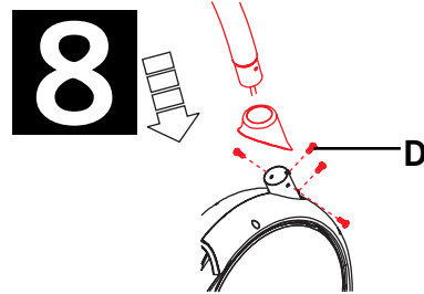
STEP 8: ATTACH CONSOLE MAST NOTE: AVOID PINCHING CONSOLE CORD
