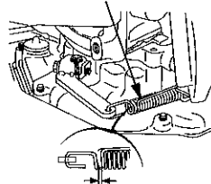
CLUTCH SPRING END
