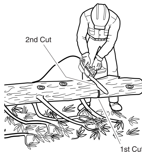
Figure 14 - Bucking Log When Log Is Supported On One End
