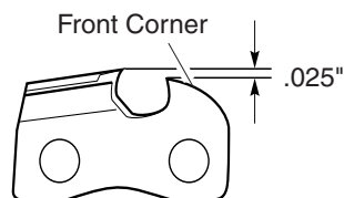
Figure 22 - Round Off Front Corner Of Depth Gauge
