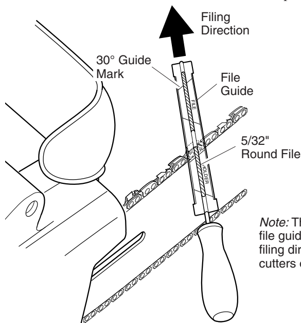
Figure 19 - File and File Guide Placement On Chain
