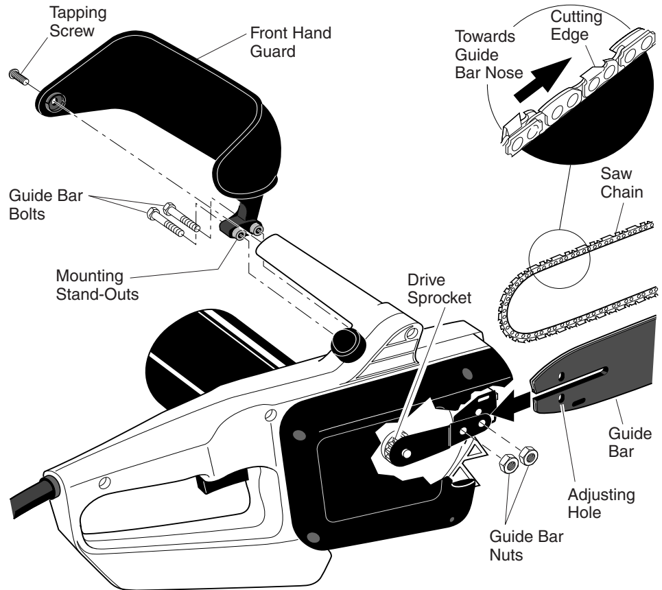
Figure 3 - Assembling Guide Bar, Chain, and Hand Guard
