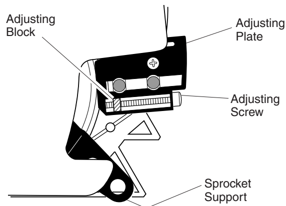
Figure 4 - Part Locations For Assembling Guide Bar
