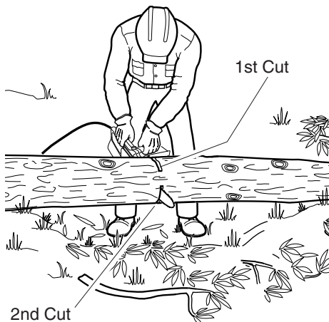
Figure 15 - Bucking Log When Log Is Supported On Both Ends
