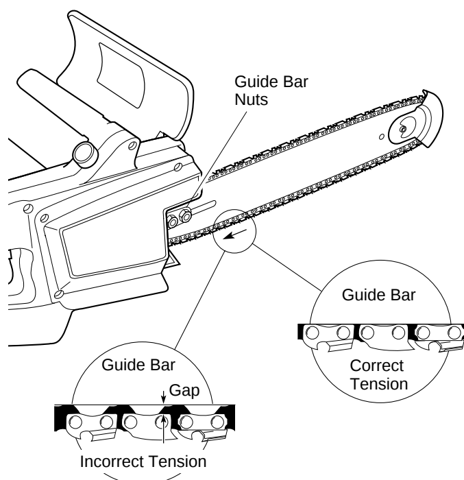
Figure 6 - Saw Chain Adjustment
