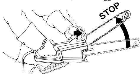
Figure 10 - The chain brake quickly stopping the saw chain
