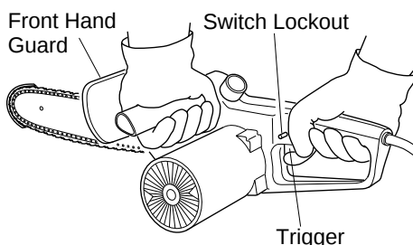
Figure 9 - Front Hand Guard, Switch Lockout, and Trigger Location
