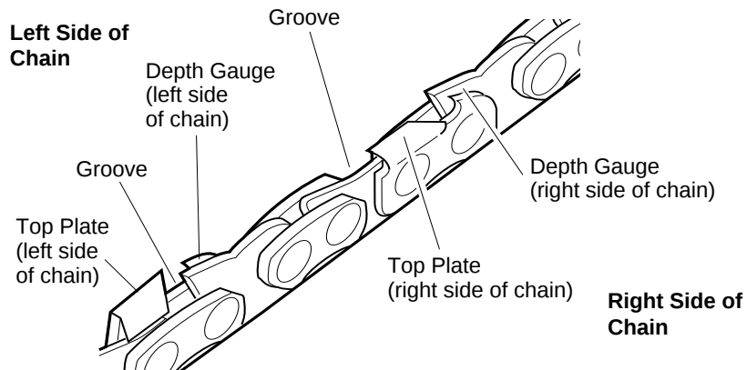
Figure 21 - Chain Part Locations
