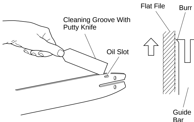
Figure 19 - Guide Bar Maintenance
