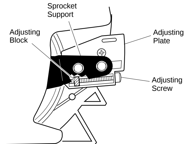
Figure 3 - Assembling Guide Bar, Chain, and Hand Guard
