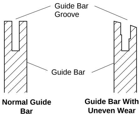
Figure 18 - Guide Bar Cross Section Showing Uneven Bar Wear
