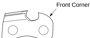
Figure 23 - Round Off Front Corner Of Depth Gauge
