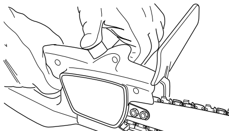
Figure 8 - Pressing Oil Cap to Oil Chain
