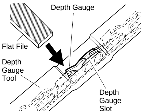
Figure 22 - Depth Gauge Tool On Chain
