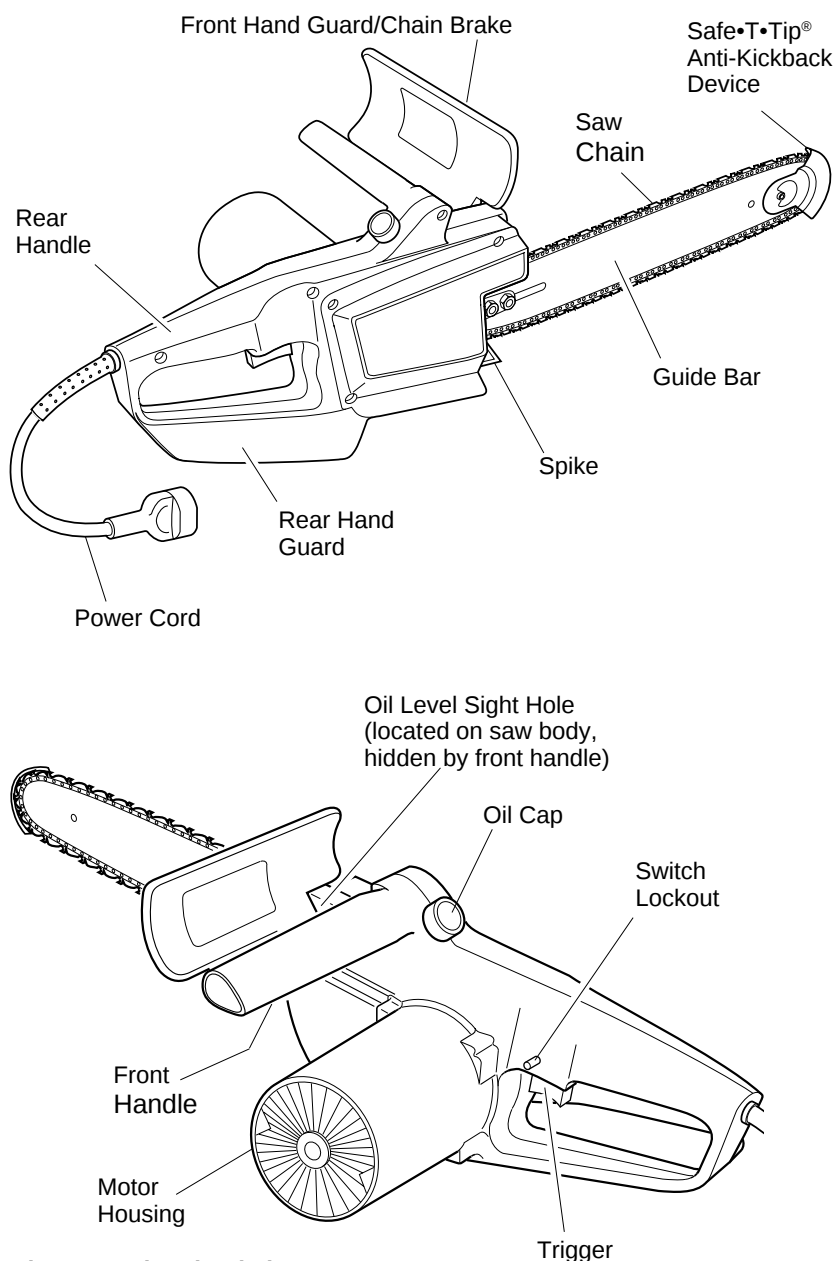
Figure 2 - Electric Chain Saw
