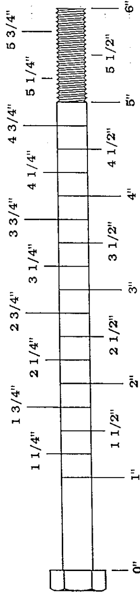
5/16" HEX BOLT
