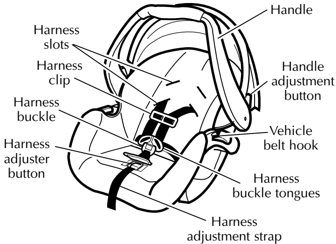
Front View: 5-Point Harness
