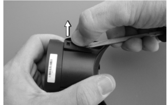
Fig. 9 – Exhaust Tee Removal - Step 1
