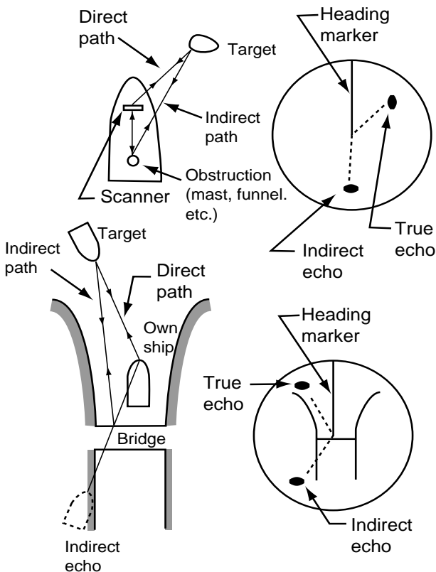
Figure 4-3 Indirect echoes
