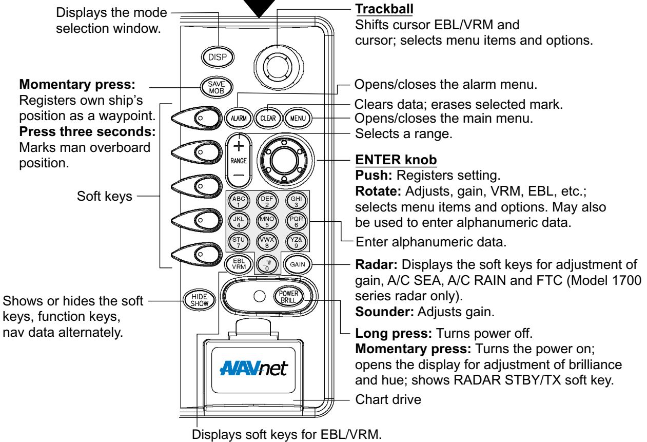
Control panel
