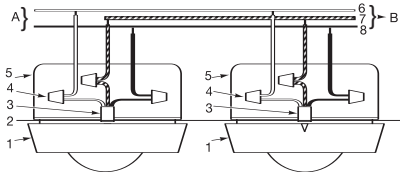
A. Unswitched 120VAC 60 Hz source B. To additional units; Maximum = 18 total (Maximum 12 Smoke Alarms)
