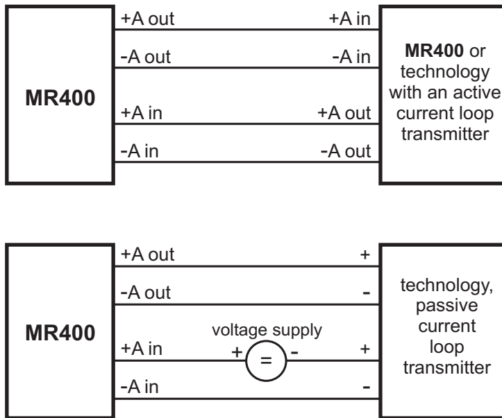
Fig. 3.7: Examples of wiring analog inputs and outputs
