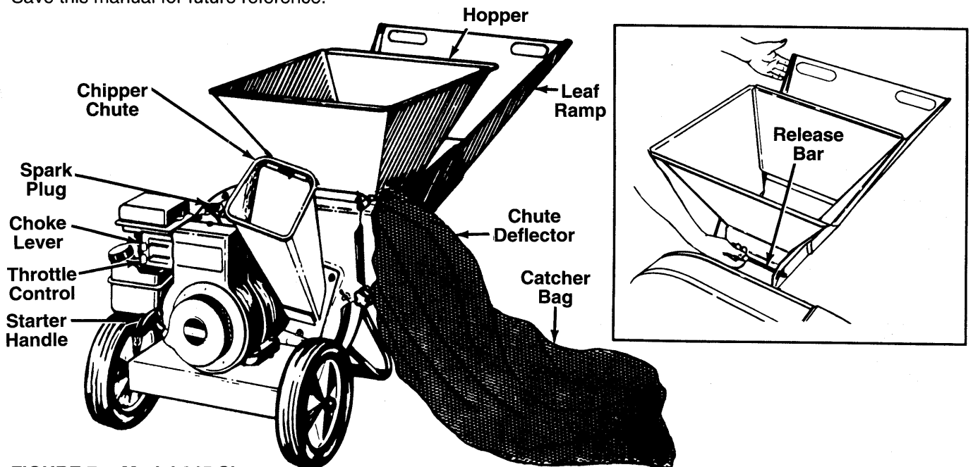
FIGURE 7.—Model 645 Shown
