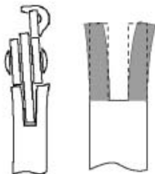
INSIDE WEAR OR SPREAD CAUSES CUTTER SIDE PLAY
