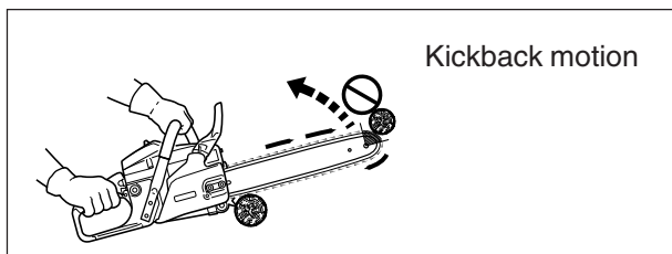
Kickback motion
