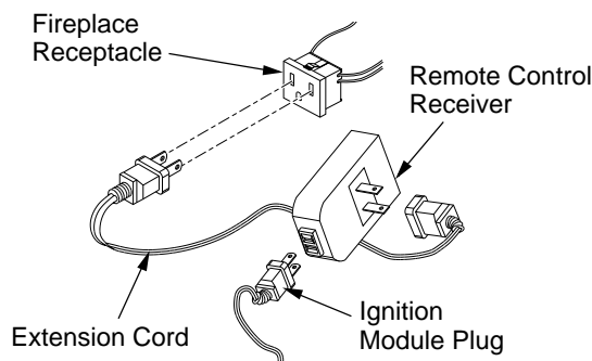
Figure 13 - Installing the WRC Remote Receiver
