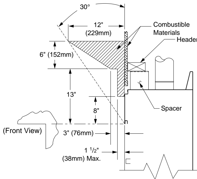
Figure 5 - Mantel Clearances - Side View (Cross Section)
