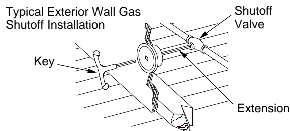
Figure 15 - Equipment Shutoff Valve Installation
