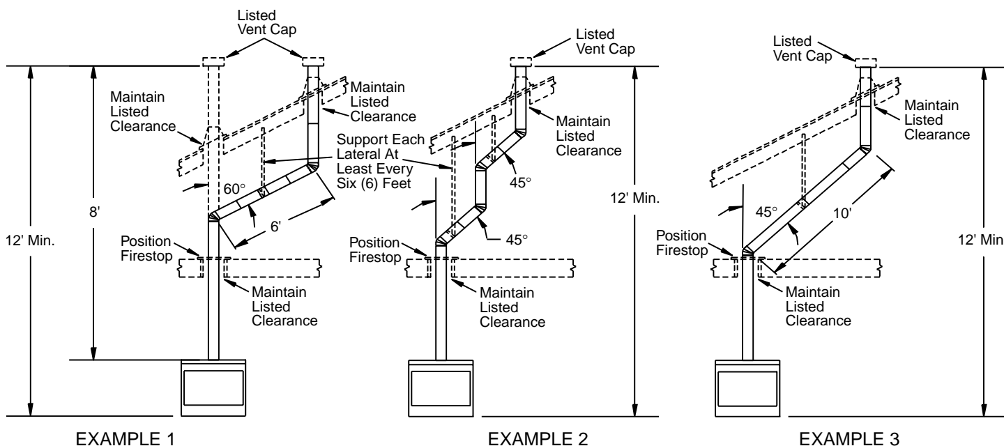
Figure 9 - Typical B-Vent Configuration
