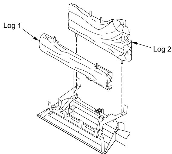
Figure 23 - Installing Logs 1 and 2
