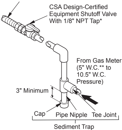
Figure 4 - Gas Connection
