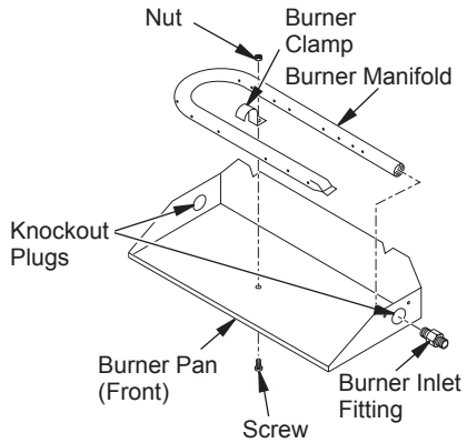
Figure 6 - Installing Burner
