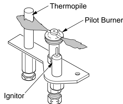
Figure 37 - Correct Pilot Flame Pattern
