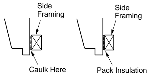
Figure 31 - Sealing Between Appliance and Framing
