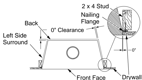
Figure 3 - Minimum Clearances (Top View)
