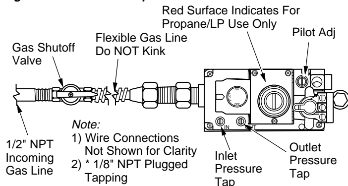
Figure 20 - Connecting Flexible Gas Line to Millivolt Valve
