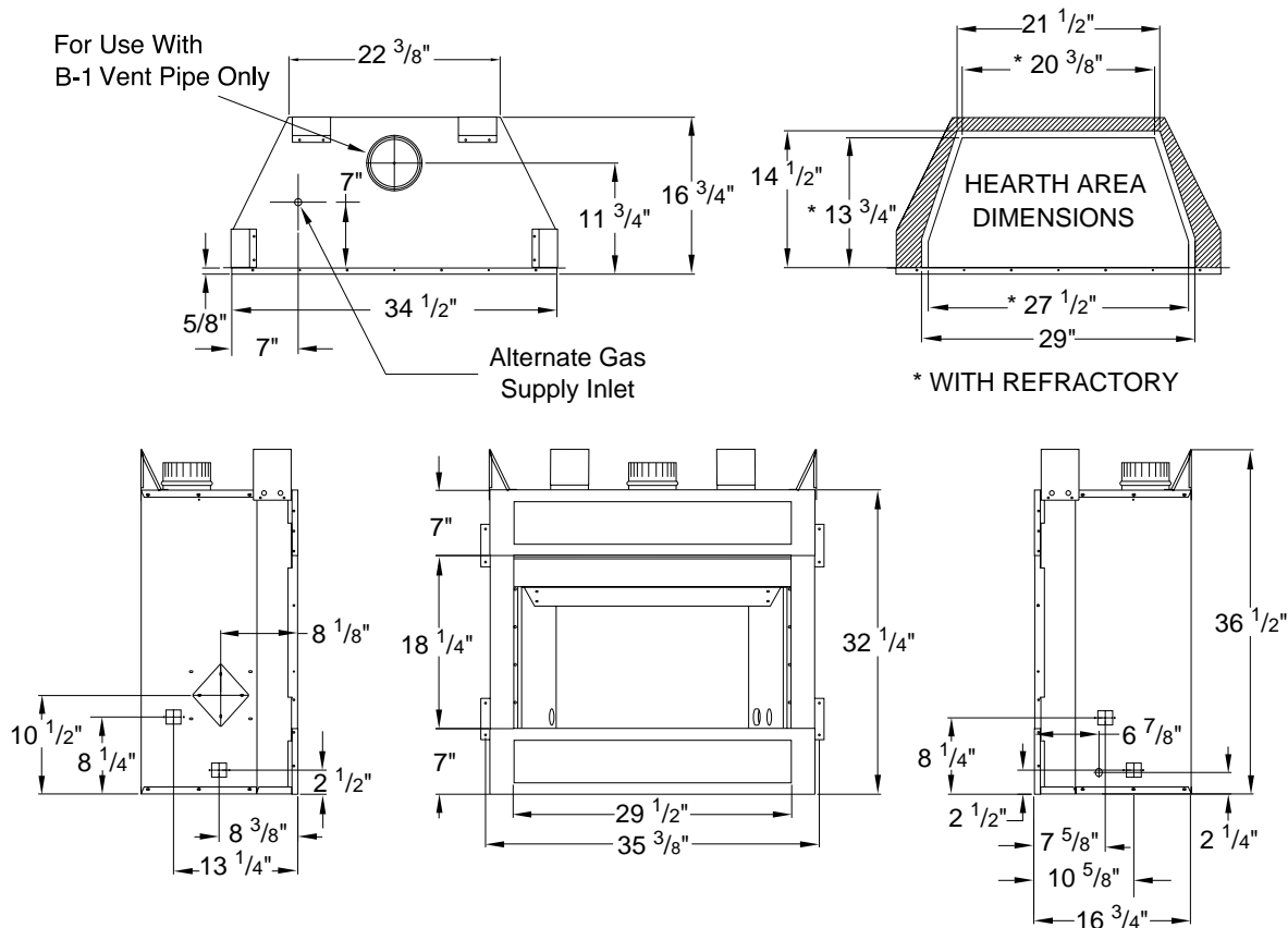
Figure 1 - Appliance Dimensions
