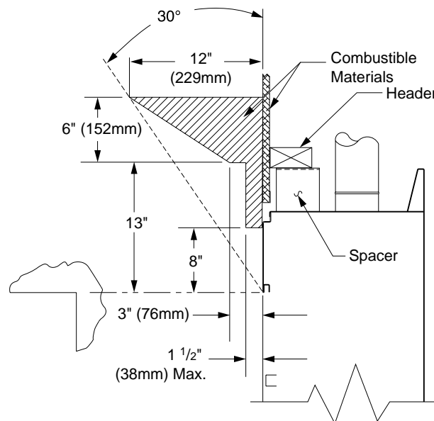
Figure 5 - Mantel Clearances - Side View (Cross Section)
