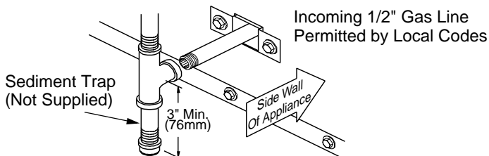
Figure 19 - Sediment Trap
