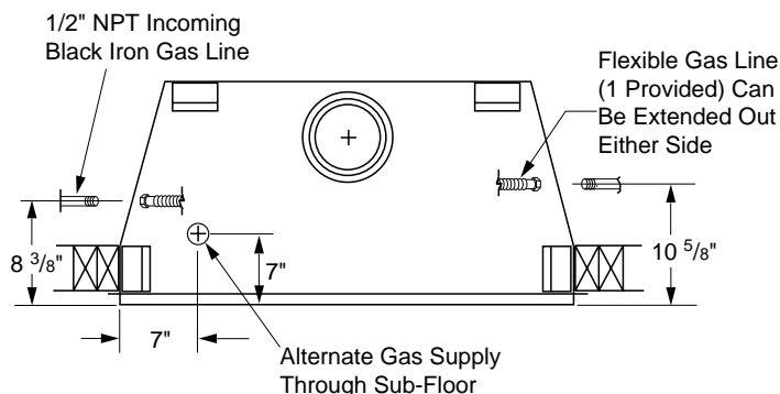
Figure 18 - Routing Incoming Gas Line
