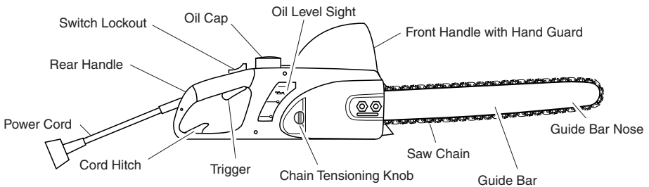
Figure 3 - Chain Saw Model 107625-01, -02, 11174-01
