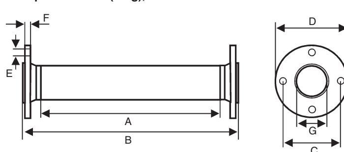
Compensateur 4" (long), 5" et 6"
