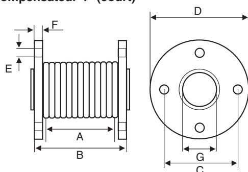
Compensateur 4" (court)
