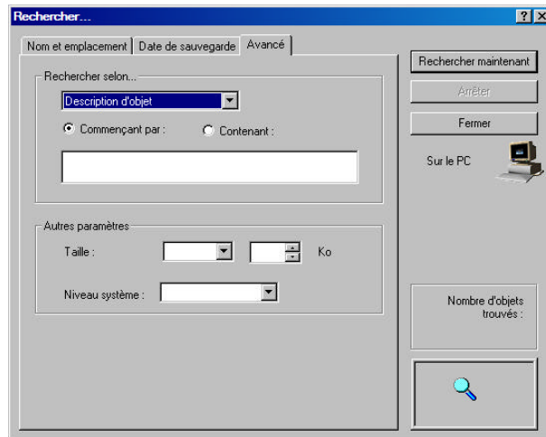
Figure 16: Onglet "Avancé"
