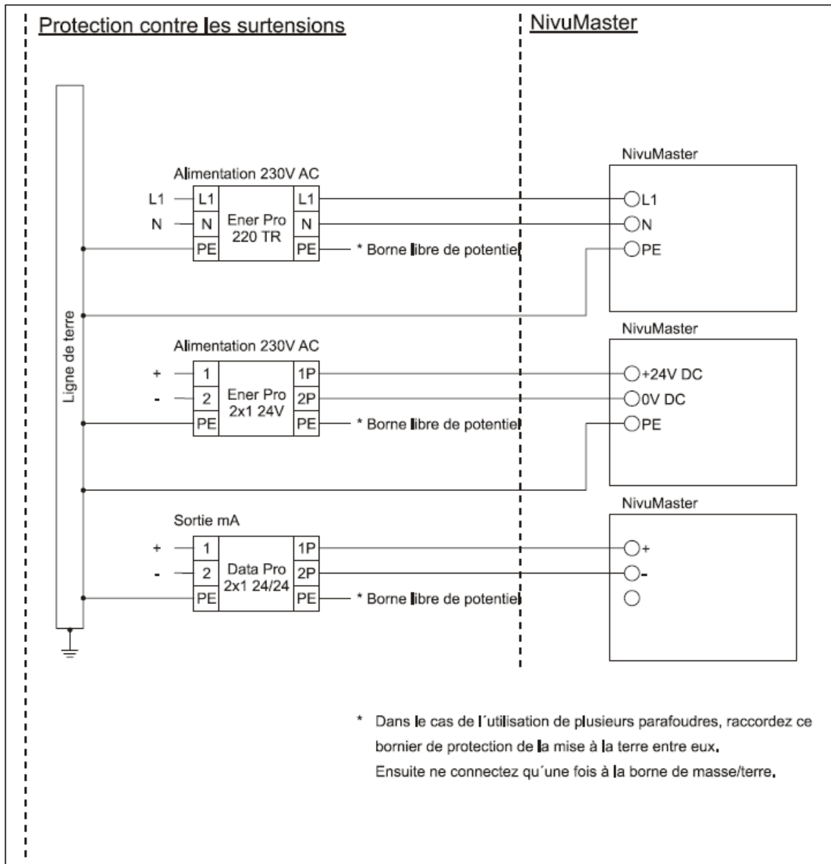
Fig. 6-6 Raccordement protection surtension
