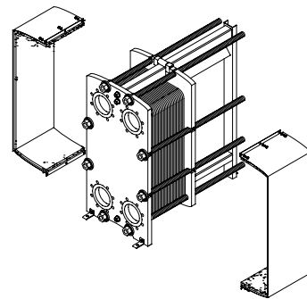
Plate pack protection with insulation mat
