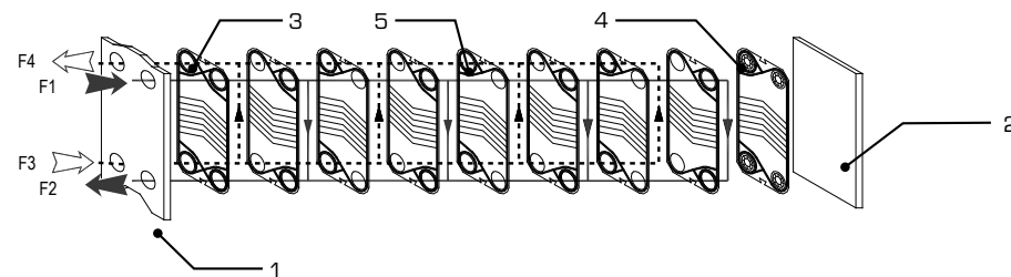
Two-pass/Two-pass arrangement (2-2)
