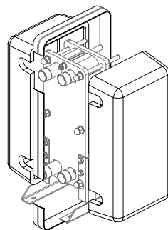
Thermoformed insulation
