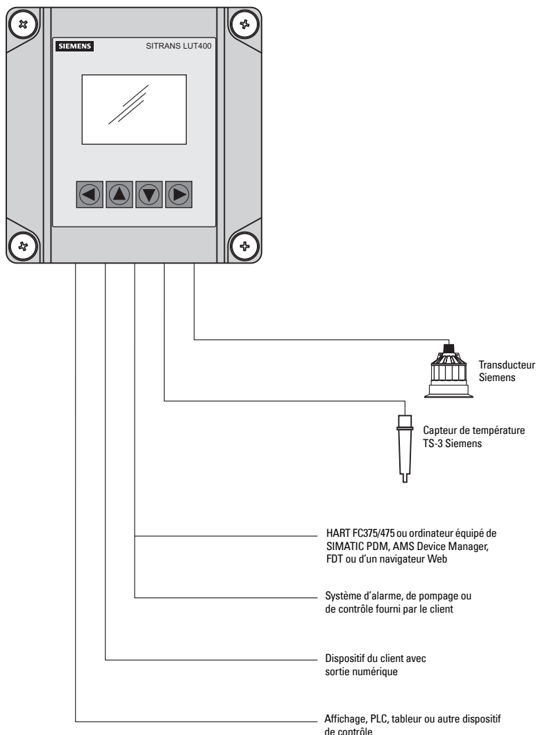
SITRANS LUT400
