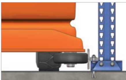
Rail de guidage.
