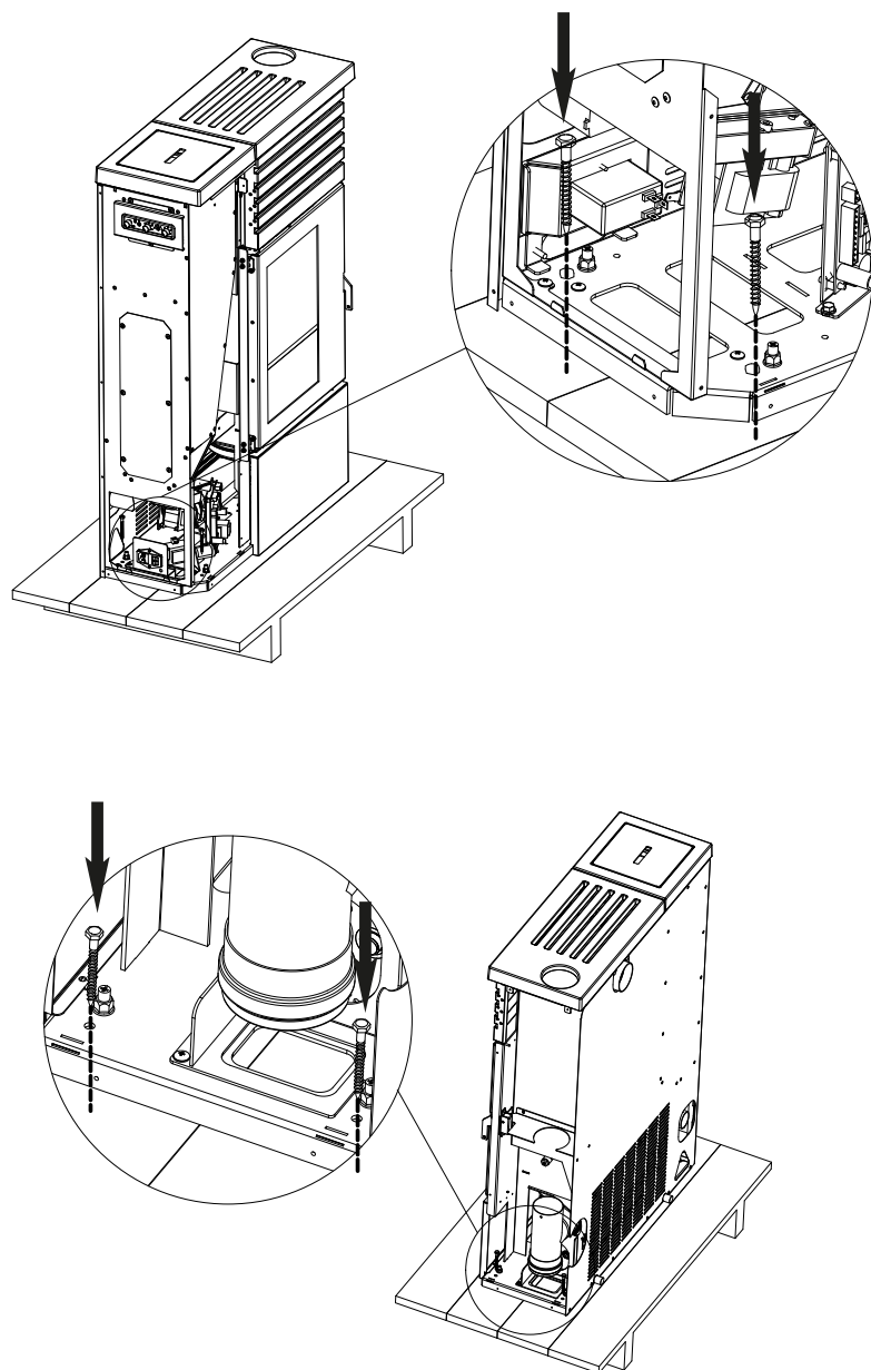
FIGURE 3 - VIS DE FIXATION EMBALLAGE POÊLE
