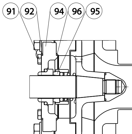
Figure 1 Garniture mécanique S1.
