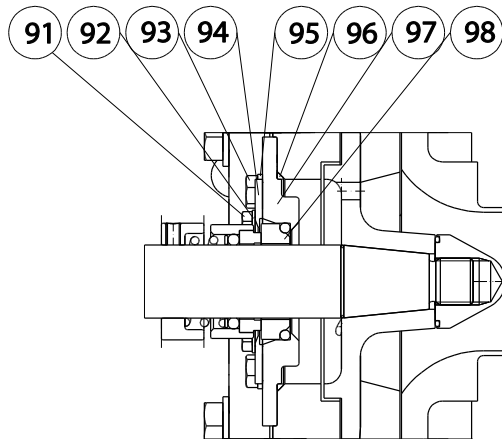
Figure 3 Garniture mécanique S12
