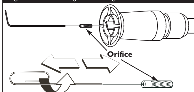
Figure 14 — Removing and Cleaning Orifice
