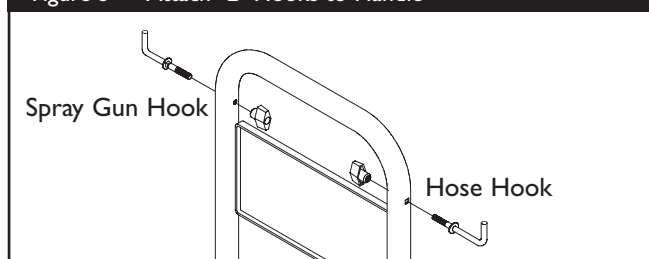
Figure 3 — Attach "L" Hooks to Handle
