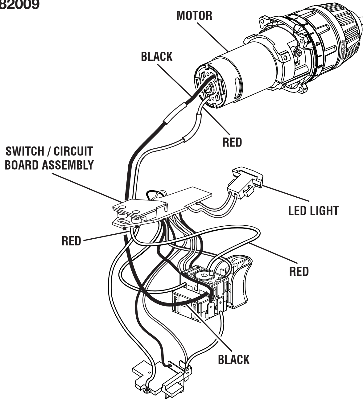
WIRING DIAGRAM
