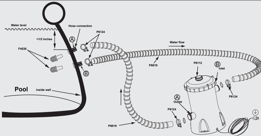
Illustration (not to scale) of pool and FlowClear™ filter-pump
