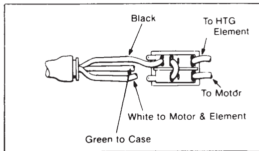
Wiring for 120V Models
