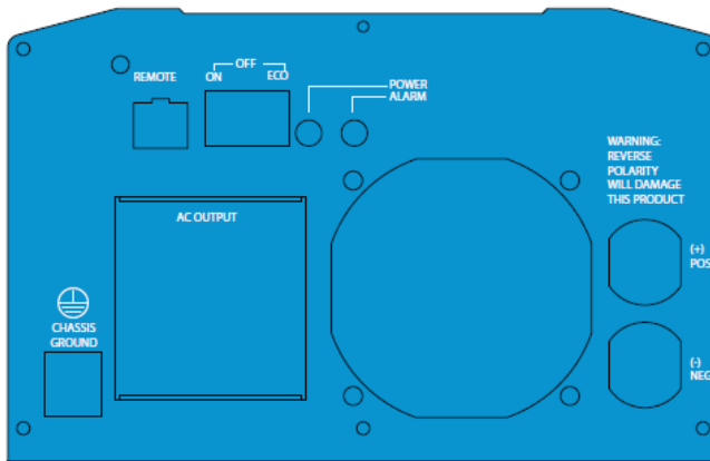
Fig 2: Front view
