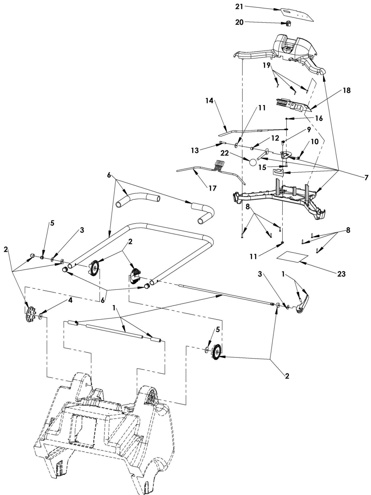
Fig. 4 – Handle Assy
