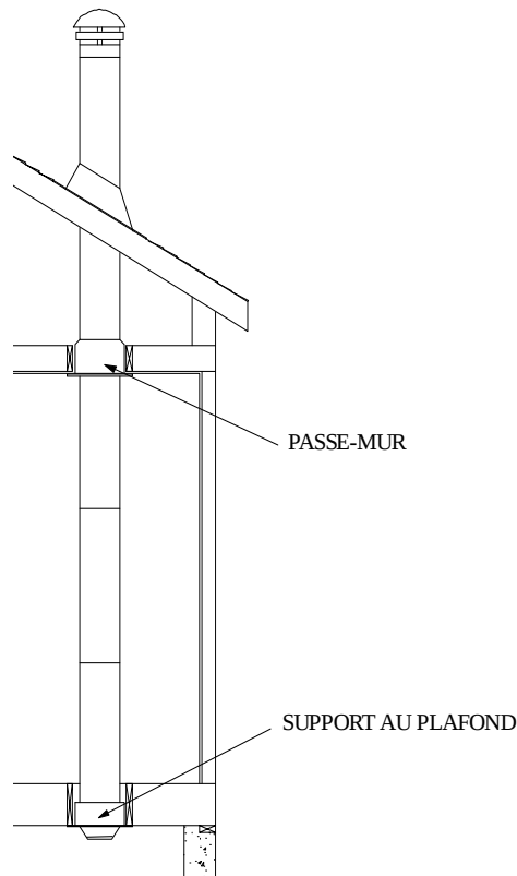
Installation verticale
