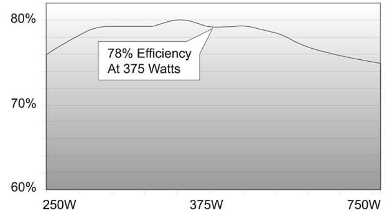
750 WATT ATX POWER SUPPLY
