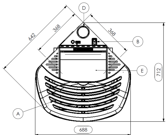
MIMOSA CAN. pellet stove dimensions
