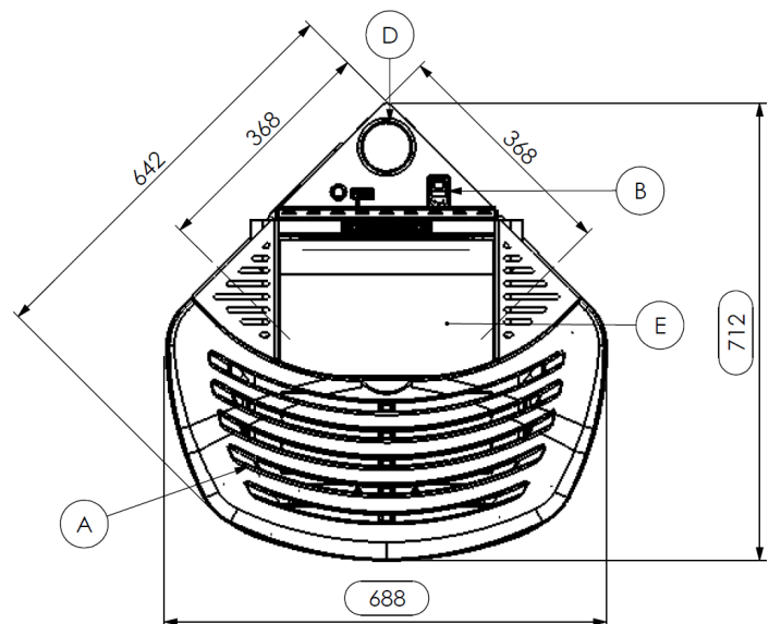
MIMOSA CAN. pellet stove dimensions
