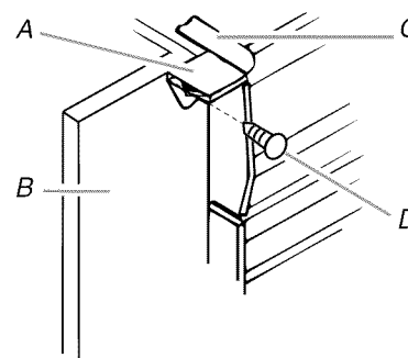
A. Mounting clip (provided) B. Kitchen cabinet C. Retaining bracket D. Mounting screw (provided)
