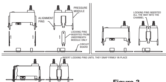
Figure 3 DCP Installation
