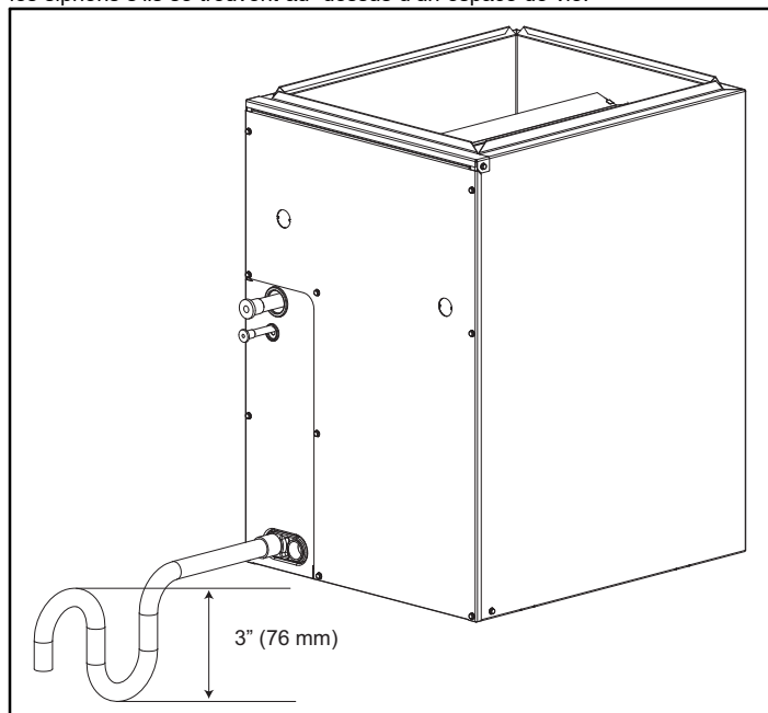
Figure 5 – Siphon de condensat
