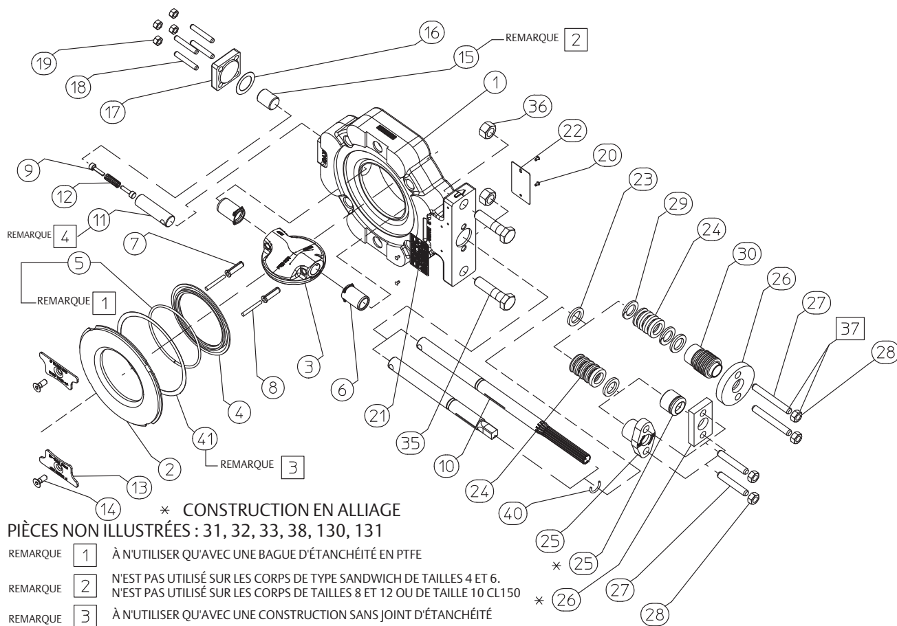
Figure 10. Vanne Fisher 8580
