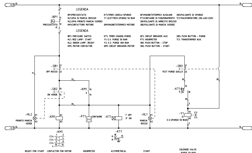
QUADRO-ELECTRICAL DIAGRAM
