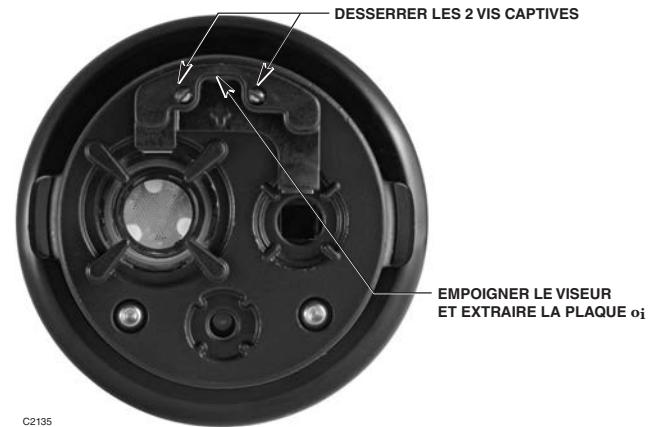
Figure 14—Extraction de la Plaque oi
