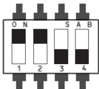
Relais/Relay/Relais / Relé/Relè 5
