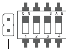
DIP switches for addressing the signal output
