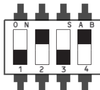
Relais/Relay/Relais / Relé/Relè 12
