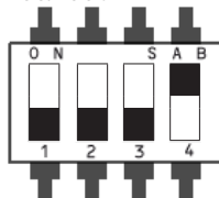
Relais/Relay/Relais / Relé/Relè 8
