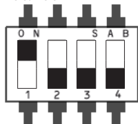
Relais/Relay/Relais / Relé/Relè 1
